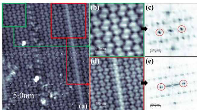
FIG. 7. (a) Large topographic image of \text{NbTe}_4 in which two smaller areas are selected and expanded. (b) Highlights the region enclosed by the green square in (a), in which no domain walls can be identified. (c) The FFT of the image in (b). No peak splitting is recognized for the (0, 2c^*/3) peaks circled in red. (d) Highlights the region enclosed by the red square in (a), in which a single domain wall can be identified. (e) The FFT of the image in (d) with a clear splitting in the (0, 2c^*/3) peaks circled in red.
