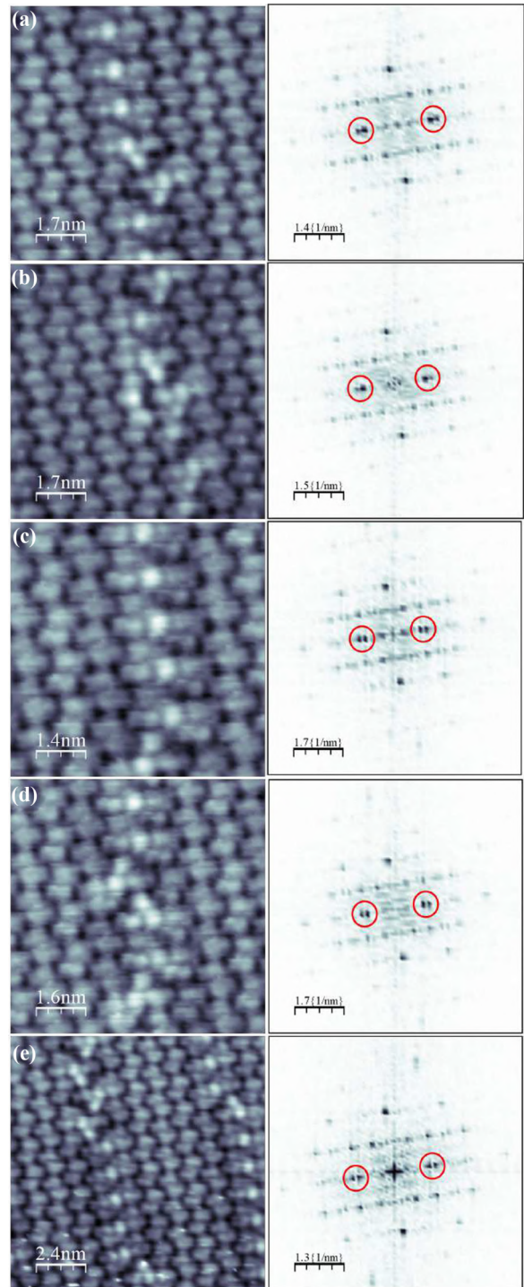
FIG. 8. Topographic images (left-column figures) around different domain walls found in our \text{NbTe}_4 samples and their corresponding FFTs (right-column figures). All FFTs show the splitting of the (0, 2c^*/3) peaks, circled in red.
