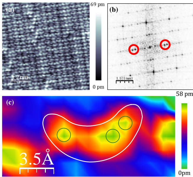
FIG. 6. (a) Topographic image of \text{NbTe}_4 in which the internal structure of the charge distribution within the cashews can be resolved. (b) FFT of the image in (a). The (0, 2c^*/3) split peaks are highlighted in red circles. (c) Expanded view of one of the cashews in (a), in which three maxima of the charge density can be clearly resolved (green circles). This is consistent with the presence of three Te atoms per cashew.
